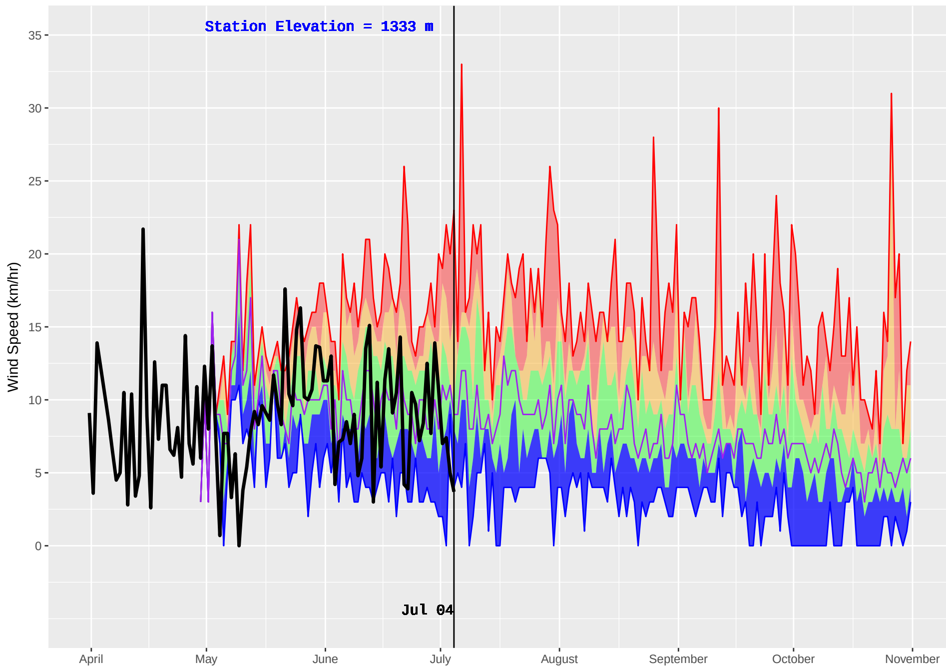
GOLDSTREAM 2 (919) : Historical (2005–2016) and Current (2018) Noon Wind Speed
