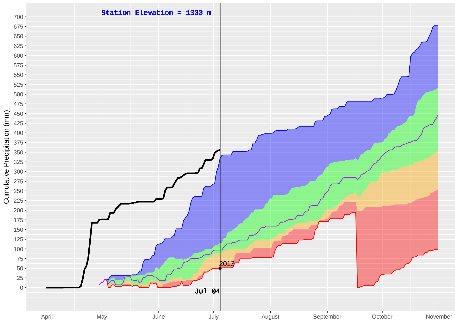
GOLDSTREAM 2 (919) : Historical (2005–2016) and Current (2018) Noon Cumulative Precipitation
